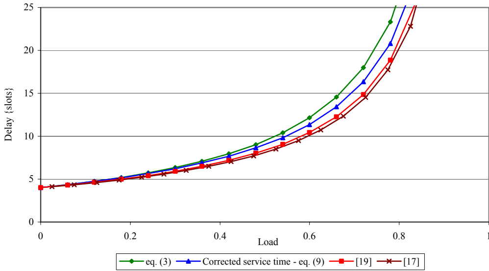
Figure 5. The exact mean access delay (obtained according to (3)), the mean access delay derived using the “corrected” service time (9), the mean access delay derived according to [19], and the mean access delay obtained according to [17] in a piconet with 4 slaves in which p_1 = p_3 = p_5 = 1/3
