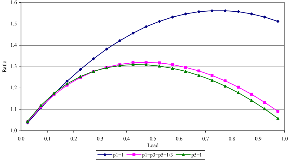
Figure 12. The ratio of the mean access delay derived according to the analysis of the exhaustive regime in [19] to the exact mean access delay (derived according to (3)) in piconets with one slave in which (1) all packets are 1 slot long, (2) the probabilities of 1, 3, and 5-slot packets are equal ( p_1 = p_3 = p_5 = 1/3 ), and (3) all packets are 5 slots long
