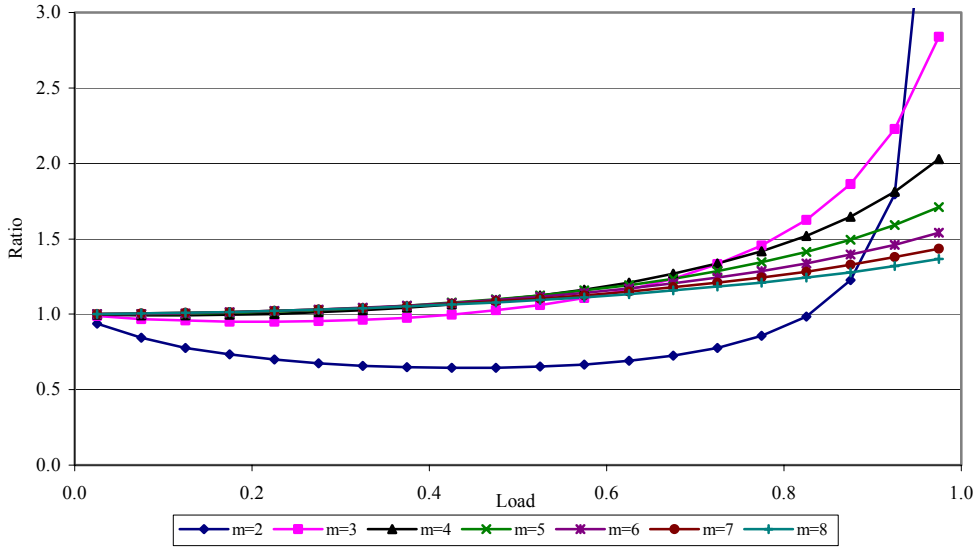
Figure 14. The ratio of the exact mean access delay (obtained according to (10)) to the mean access delay derived according to [20] in piconets with only uplink traffic operated in the exhaustive regime in which the probabilities of 1, 3, and 5-slot packets are equal ( p_1 = p_3 = p_5 = 1/3 )
