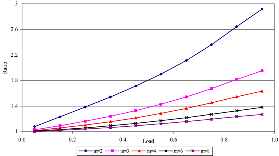
Figure 7. The ratio of the exact mean access delay (obtained according to (3)) to the mean access delay derived according to [19] in piconets in which all packets are 5 slots long ( p_5 = 1 )
