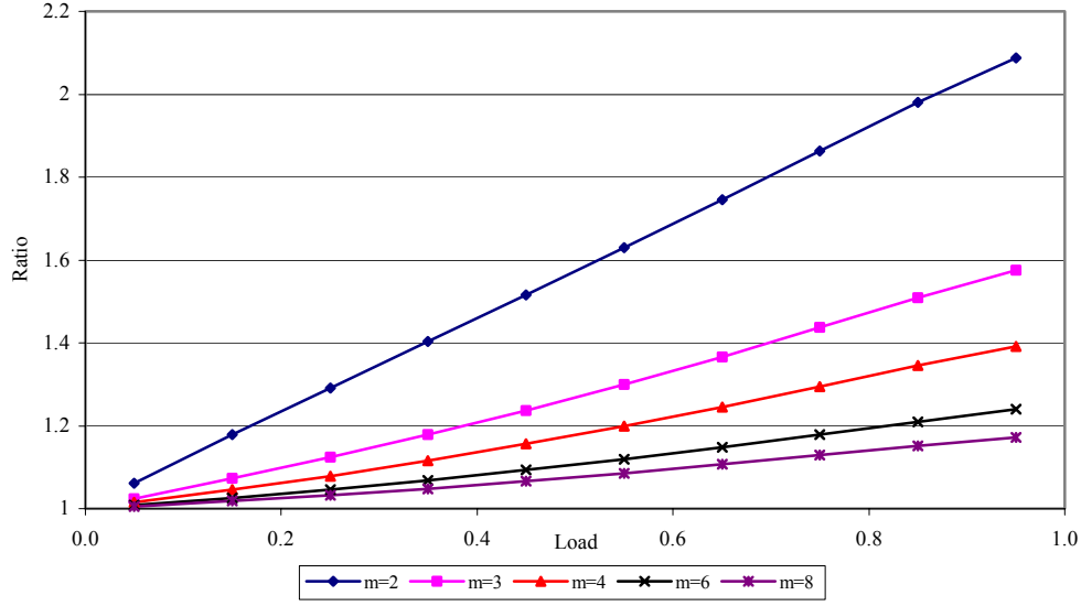
Figure 6. The ratio of the exact mean access delay (obtained according to (3)) to the mean access delay derived according to [19] in piconets in which p_1 = p_3 = p_5 = 1/3
