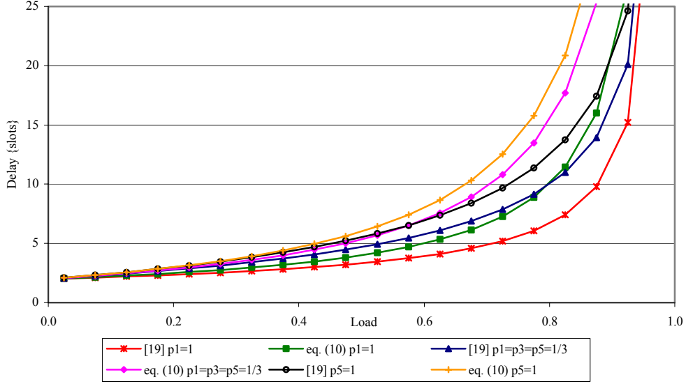
Figure 13. The mean access delay derived according to [19] and the exact mean access delay (derived according to (10)) in piconets with only uplink traffic operated in the exhaustive regime. The piconets are composed of 2 slaves and the packets are 1 slot long, 1, 3, and 5 slots long with equal probability ( p_1 = p_3 = p_5 = 1/3 ), and 5 slots long
