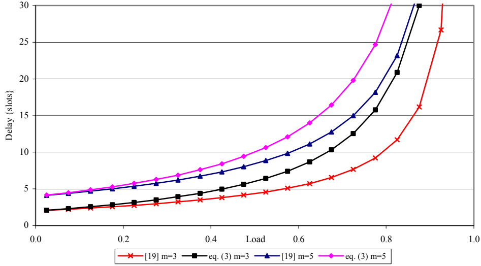
Figure 4. The mean access delay derived according to [19] and the exact mean access delay (computed according to (3)) in piconets with 2 and 4 slaves in which all packets are 5 slots long
