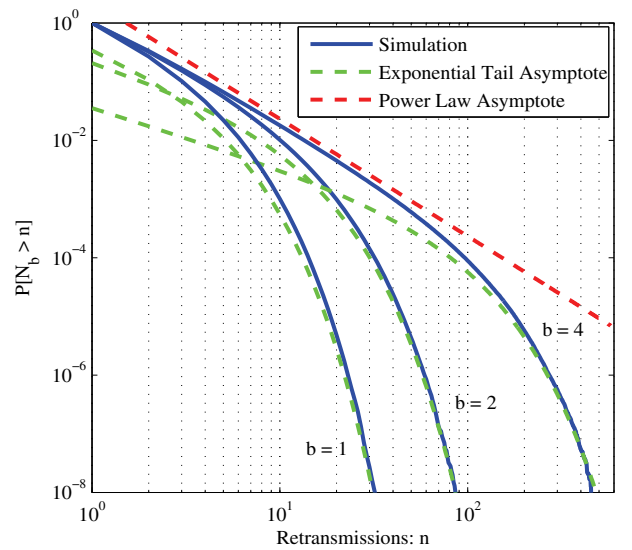
Figure 4: Example 2. Exponential tail asymptotics.
