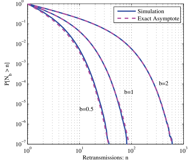
Figure 3: Example 1(b). Exact asymptotics for \alpha < 1 .
