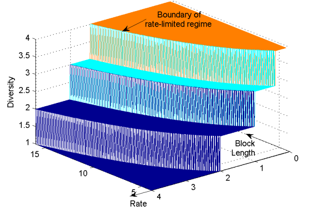
Fig. 5. The tradeoff between diversity, rate, and block length for MMSE SC-FDE.
