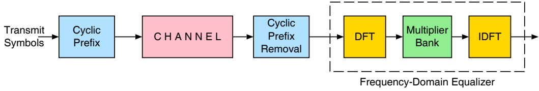
Fig. 1. Block diagram of a SC-FDE system.
