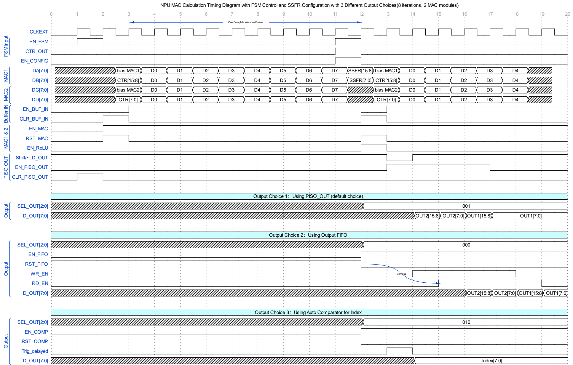
Figure 6. Recommended operation timing diagram
