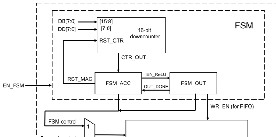
Figure 4. Block diagram of FSM
