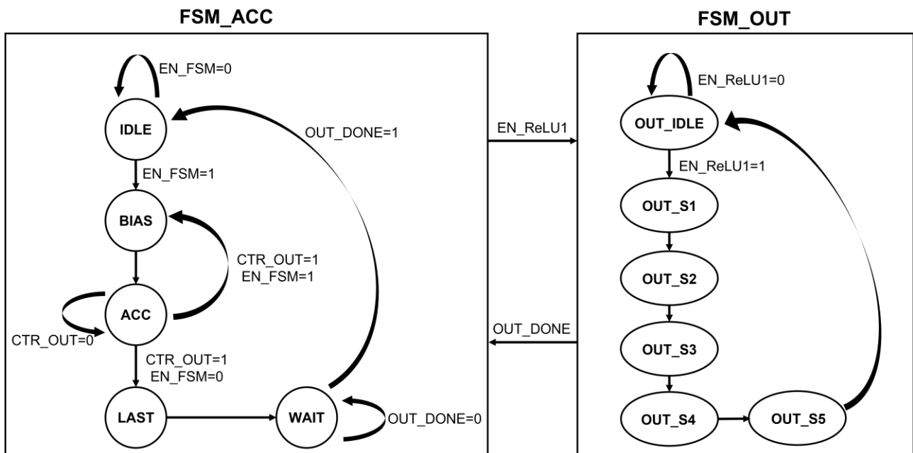
Figure 5. State transition diagram of FSM_ACC and FSM_OUT
