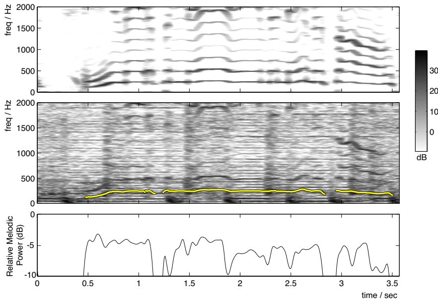
Figure 3.1: Examples from training data generation. The fundamental frequency of the isolated melody track (top pane) was estimated and time-aligned to the complete audio mix (center). The fundamental frequency estimates, rounded to the nearest semitone were used as target class labels (overlaid on the spectrogram). The bottom panel shows the power of the melody voice relative to the total power of the mix (in dB); if the mix consisted only of the voice, this would be 0 dB.
