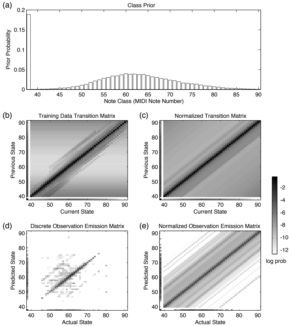
Figure 3.5: Hidden Markov parameters learned from the ground truth and confusion matrix data. Top (pane (a)): class priors. Middle: state transition matrix, raw (pane (b)), and regularized across all notes (pane (c)). Bottom: Observation likelihood matrix for the discrete-label smoothing HMM, raw (pane (d)) and regularized across notes (pane (e)).
