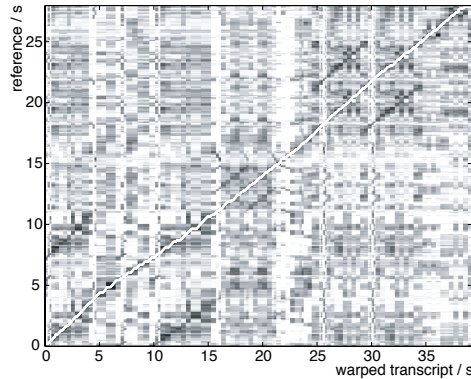
Figure 6.2: Similarity matrix calculated between an audio recording and a MIDI rendition of Tchaikovsky’s January: At the Fireside from The Seasons . Dark regions indicate similarity between the feature matrices, and the least-cost path warping estimate is overlaid in white.
