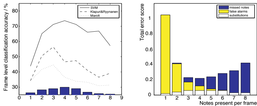
Figure 4.5: Left: Variation of classification accuracy with number of notes present in a given frame and relative note frequency. Right: Error score composition as a function of the number of notes present.
