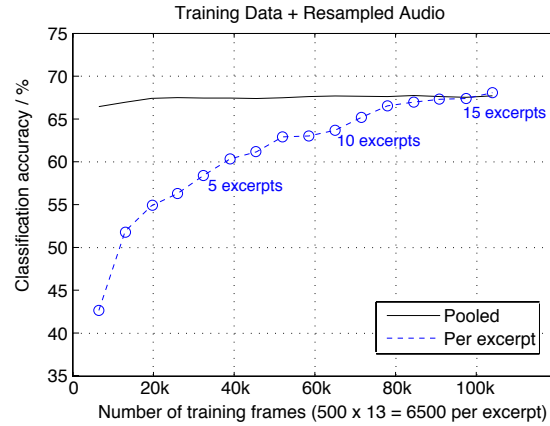
Figure 3.3: Variation of classification raw pitch accuracy with the total number of excerpts included, compared to sampling the same total number of frames from all excerpts pooled. This data set includes 13 resampled versions of each excerpt, with 500 frames randomly sampled from each transposition.
