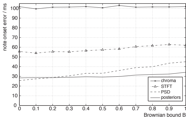
Figure 6.3: Time warp mean onset errors.
