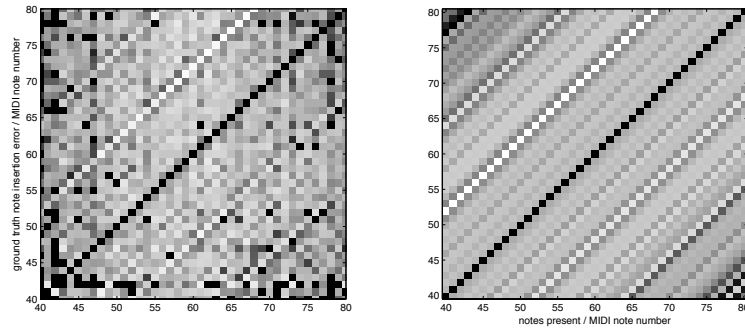
Figure 7.1: Left: Log-probability note accompaniment occurrence for note insertion errors. Right: Log-probability note accompaniment insertion errors normalized by averaging along the diagonals of the matrix in order to facilitate generalization.
