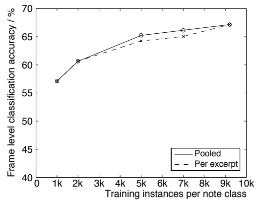
Figure 4.3: Variation of classification accuracy with the total number of excerpts included, compared to sampling the same total number of frames from all excerpts pooled.
