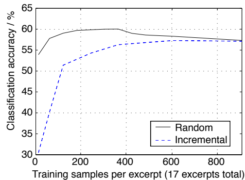
Figure 3.2: Variation of classification accuracy with number of training frames per excerpt. Incremental sampling takes frames from the beginning of the excerpt; random sampling takes them from anywhere. The training set does not include resampled (transposed) data.
