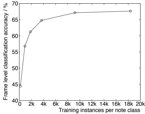
Figure 4.2: Variation of classification accuracy with number of randomly selected training frames per note, per excerpt.
