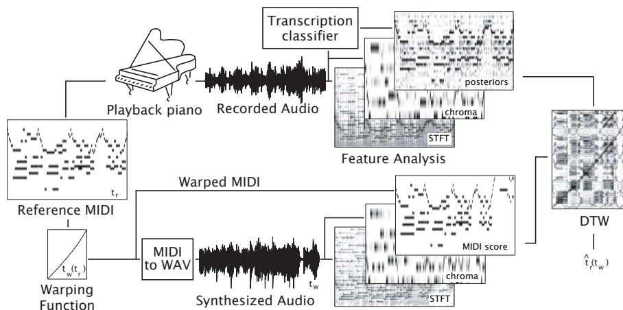
Figure 6.1: Flow chart of the data generation and feature analysis for score to audio alignment.
