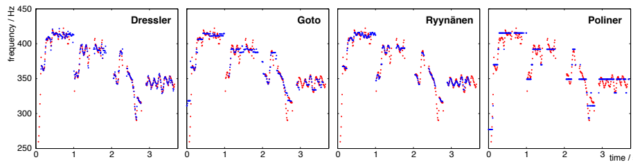
Figure 3.7: Examples of melody transcription estimations from several of the submitted systems as compared to the ground truth (light dots) for a 3.7 s excerpt from “Frozen” by Madonna.
