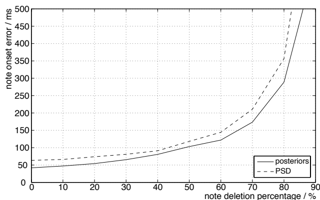
Figure 6.5: Note deletion mean onset errors for the linearly scaled test cases.
