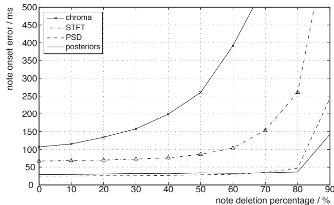
Figure 6.4: Note deletion mean onset errors.
