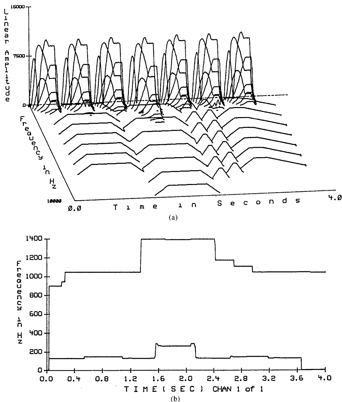
Fig. 14. Artificial duet example 2. (a) Raw MQ analysis. (b) TWM duet frequency-tracking results.
