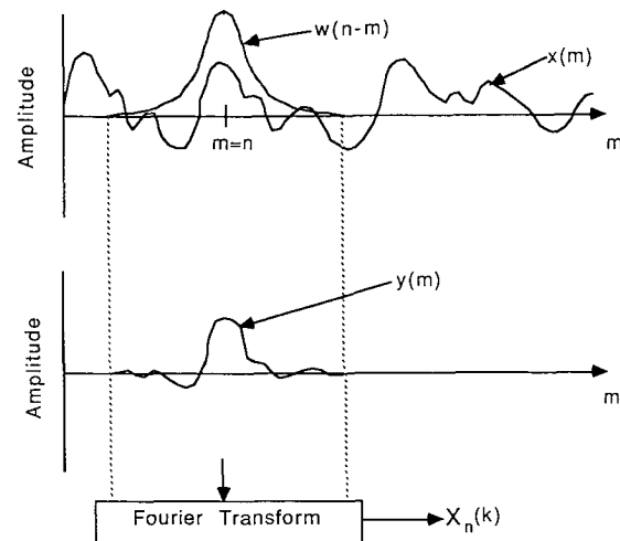
Fig. 1. The Fourier transform viewpoint of STFT. A segment of the digitized signal x(m) is multiplied by the reversed and shifted window function w(n-m) . The resulting signal y(m) is processed by the discrete Fourier transform.
