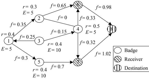
Figure 1. The required transmission rates ( r_i ), the initial energy values ( E_i ), and the optimal flows ( f_{ij} ) in a network of badges (assuming that e_i = 1 \forall i )
