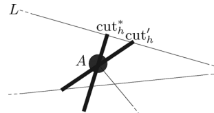
Fig. 14. Translate an endpoint of \text{cut}_h^* along L until it can no longer intersect the bottom link. This new cut is \text{cut}'_h .
