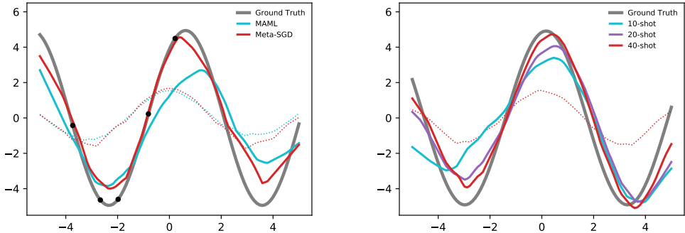
Figure 3: Left: Meta-SGD vs MAML on a random 5-shot regression task. Both initialization (dotted) and result after one-step adaptation (solid) are shown. Right: Meta-SGD (10-shot meta-training) performs better with more training examples in meta-testing.
