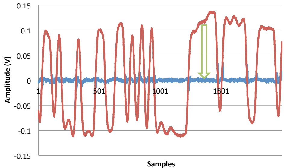
Fig 4. Time domain analysis before/after digital cancellation in the baseband.
