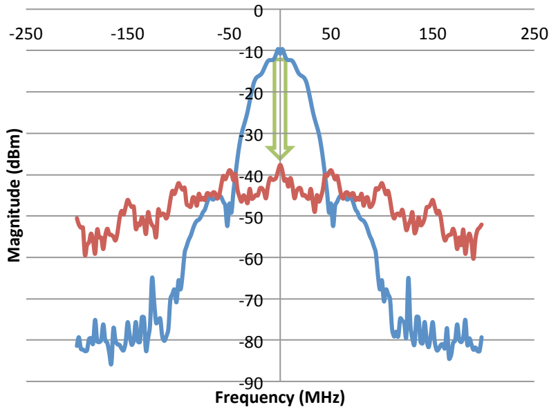
Fig 3. Spectrum analysis before/after digital cancellation in the baseband.
