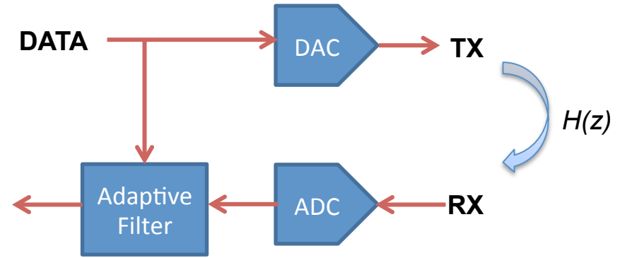
Fig 2. Adaptive filter generates its coefficients as close as possible to H(z) based on LMS algorithm with the received signal and the reference data signal.
