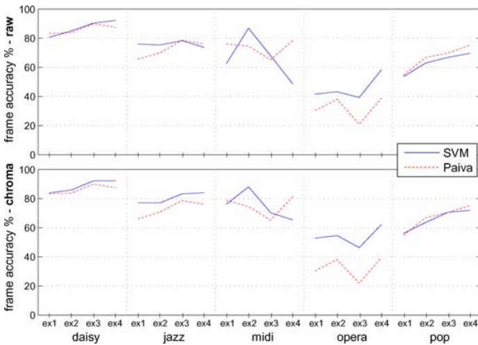
Fig. 4 Variation in voiced transcription frame accuracy across the 20 excerpts of the ADC 2004 evaluation set (4 examples from each of 5 genre categories, as shown). Solid line shows the classification-based transcriber; dashed line shows the results of the best-performing system from the 2004 evaluation. Top pane is raw pitch accuracy; bottom pane folds all results to a single octave of 12 chroma bins, to ignore octave errors
