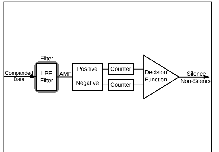
Fig. 7. Block diagram of proposed algorithm
