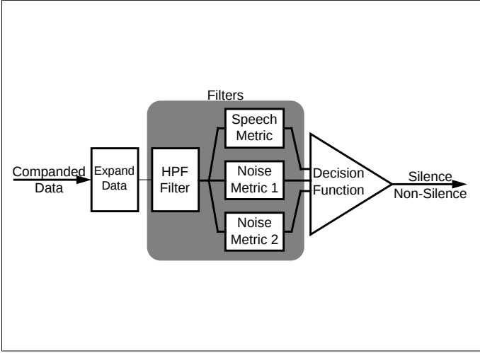
Fig. 1. Block diagram of Savoji algorithm
