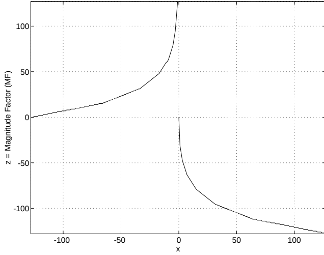
Fig. 4. Composite function
