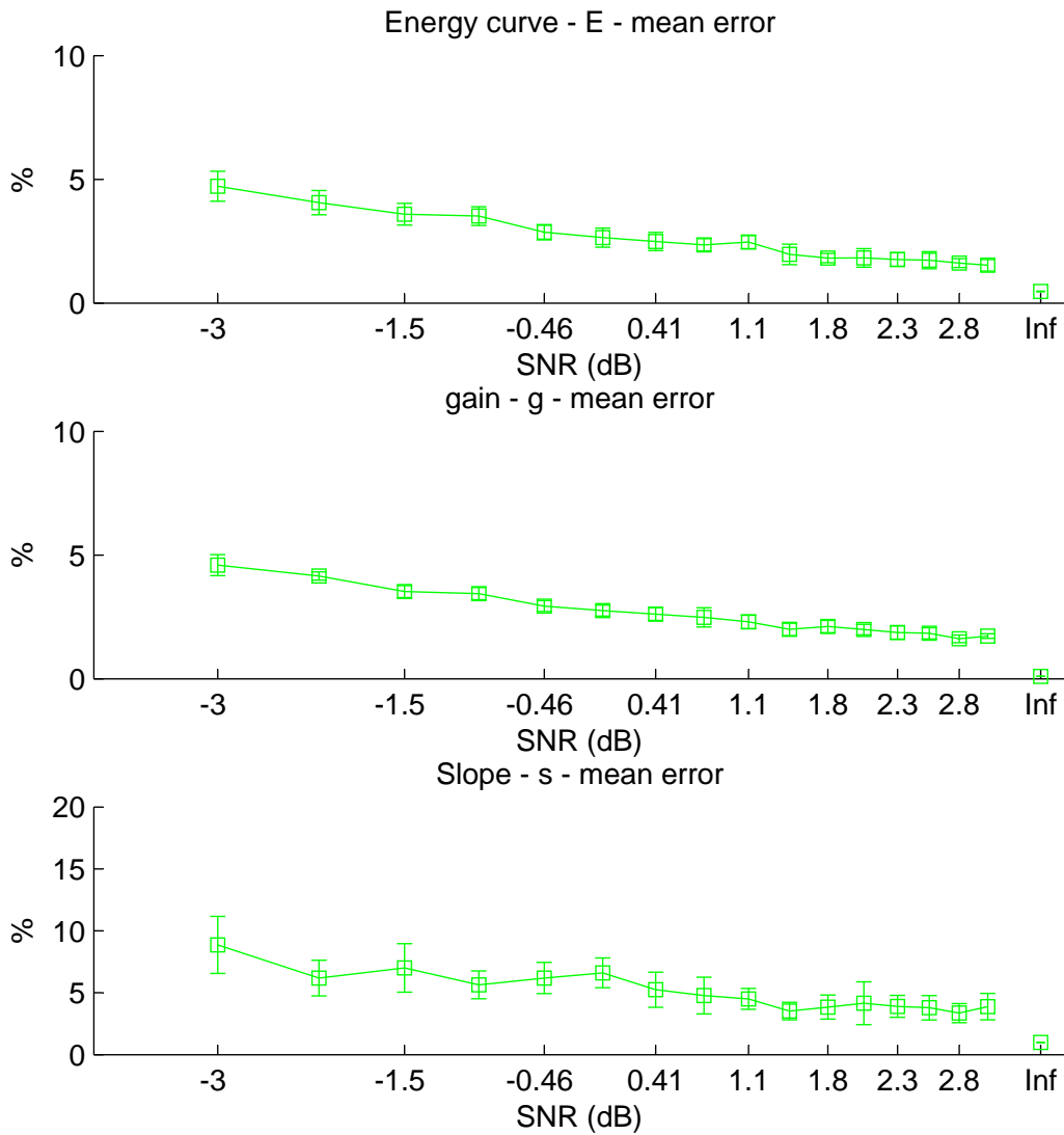
Figure 8.10: Plots of the mean error of the parameters of the linear model. The mean is take across all iterations, all harmonics ( g_i, s_i ) or all time points ( E ) relative to the square root of the mean square of the true values. The error bars represent the standard deviation in this mean calculated across iterations.
