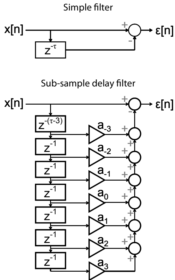
Figure 4.2: Optimal cancellation filters. Top: for signals with integer periodicities; bottom: a filter able to cancel non-integer periodicities.
