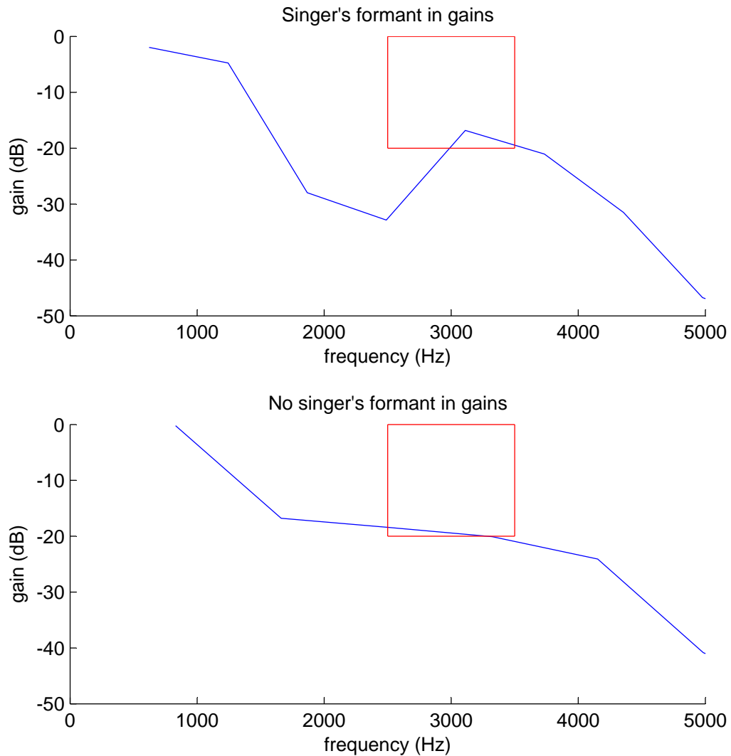
Figure 9.7: Singer's formant examples. Both plots show the gains associated with notes from The Pirates of Penzance . The red boxes outline the region where there needs to be a peak in the gains in order for the note to have the singer's formant. The top plot shows the gains associated with a single note that shows evidence of the singer's formant and the bottom plot shows gains associated with a single note that does not.
