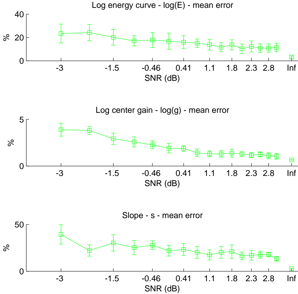
Figure 8.4: Plots of the mean error of the parameters of the log model. The mean is taken across all iterations, all harmonics ( g_c, s ) or all time points ( E ) relative to the square root of the mean square of the true values. The error bars represent the standard deviation in this mean calculated across iterations.
