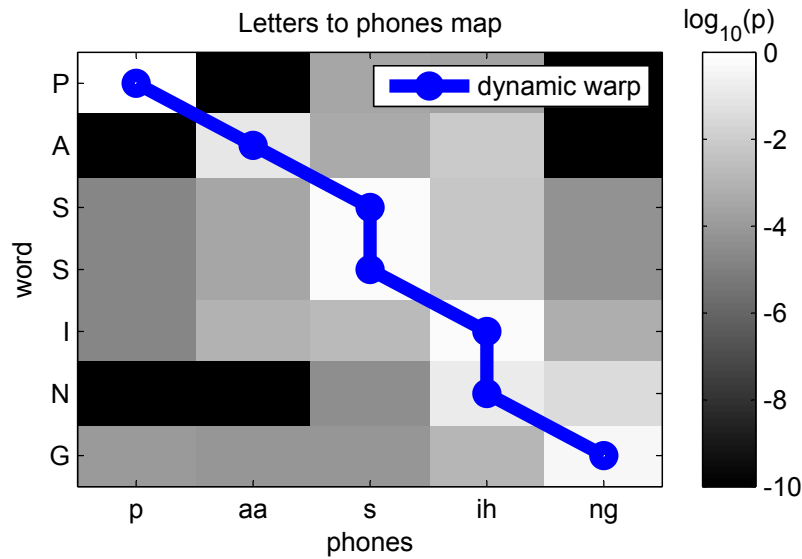
Figure 3.2: Mapping ‘passing’ to ‘p aa s ih ng’. The letter-to-phones probability map for ‘passing’ and ‘p aa s ih ng’ is generated by taking the appropriate columns and rows from the converged alphabet-to-phones map (figure 3.1, bottom plot). The line shows the results of the dynamic warp. Once again, the probabilities are shown in the log scale.
