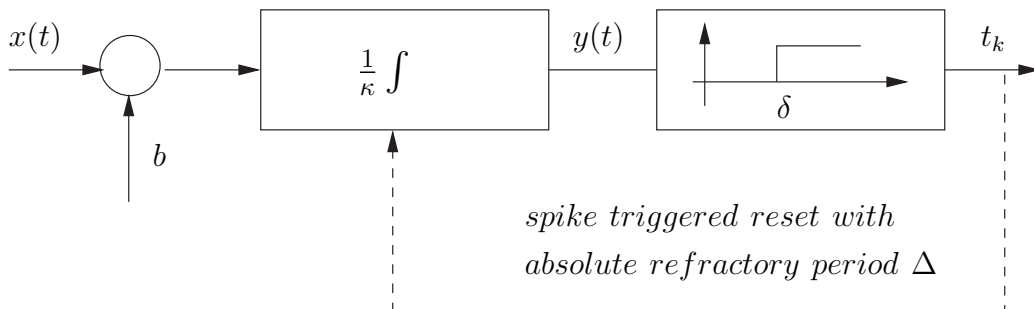
Figure 1: Time Encoding with the Integrate-and-Fire Neuron.
