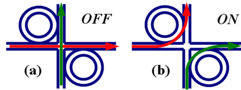
Figure 2. Photonic switching element: (a) OFF state: a passive waveguide crossover. (b) ON state: light is coupled into rings and forced to turn
