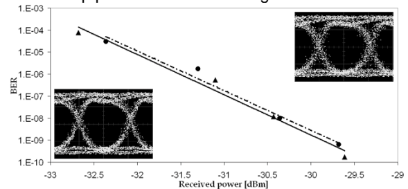
Fig. 4 – BER curves for the module after 1 hop (●,dashed), and back-to-back (▲,solid) indicate a power penalty < 0.2dB. Eye diagrams at 10 Gb/s ( \lambda=1554.4 nm) for back-to-back (bottom left) and after 3 loop passes (top right).
