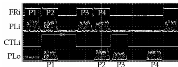
Fig. 3 – The waveforms shown are (top down): input frame optical signal, input payload, input control signal, and output payload (after a latency of 38 ns). Four packets, annotated P1 through P4, are injected into the module and only proceed to the output when the control signal is low.
