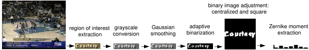
Fig. 3. Processing steps for Zernike moment extraction.
