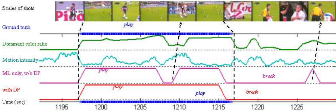
Fig. 3. Part of clip Argentina (19’52” 20’30”): key frames, feature contours, and segmentation results (with or without dynamic programming)
