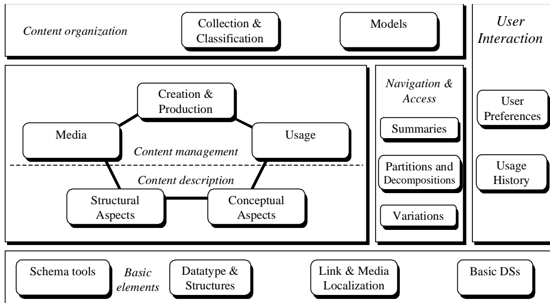
Figure 4: Overview of MPEG-7 Multimedia Description Schemes
