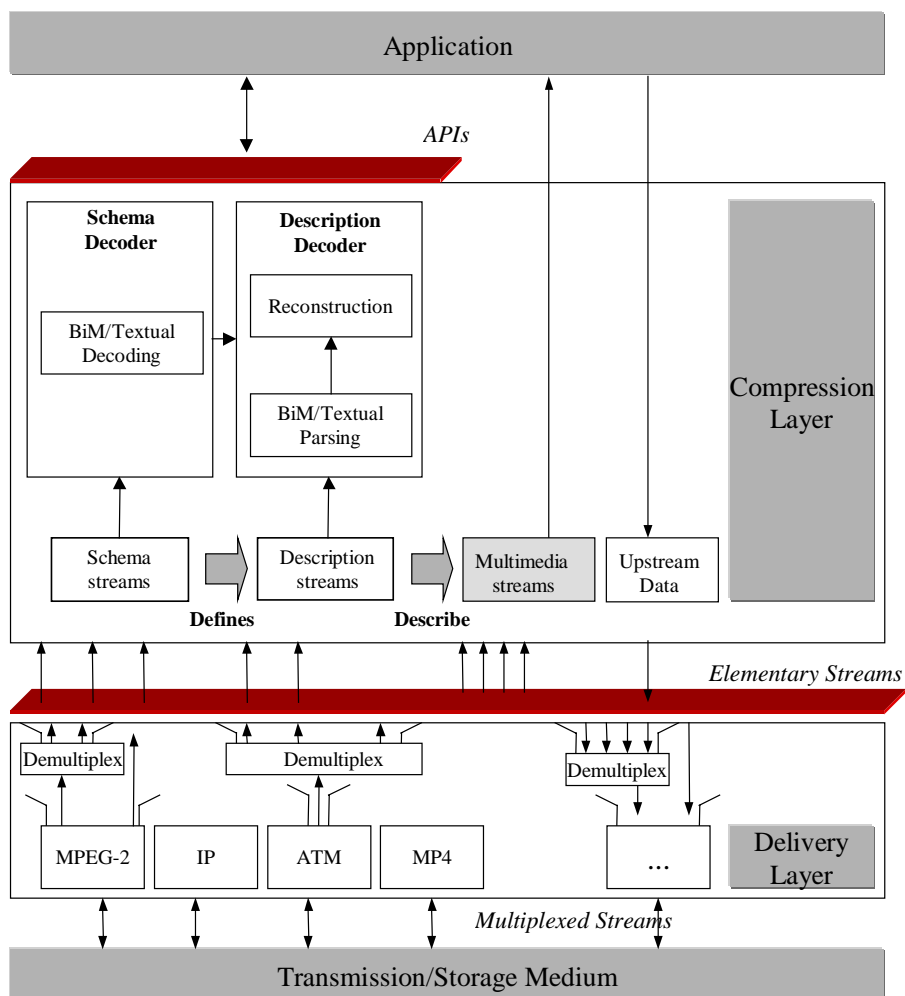
Figure 3: Architecture of MPEG-7 Terminal
