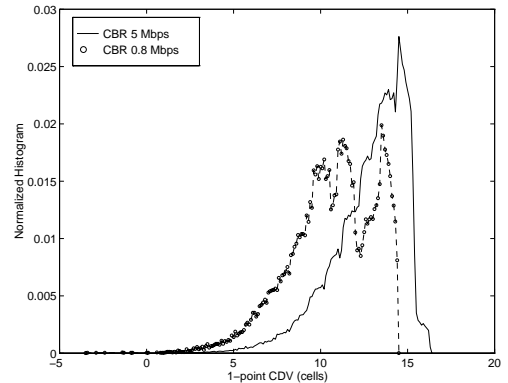
Figure 2: 1-point CDV Normalized Histogram for Scenario CBR.
